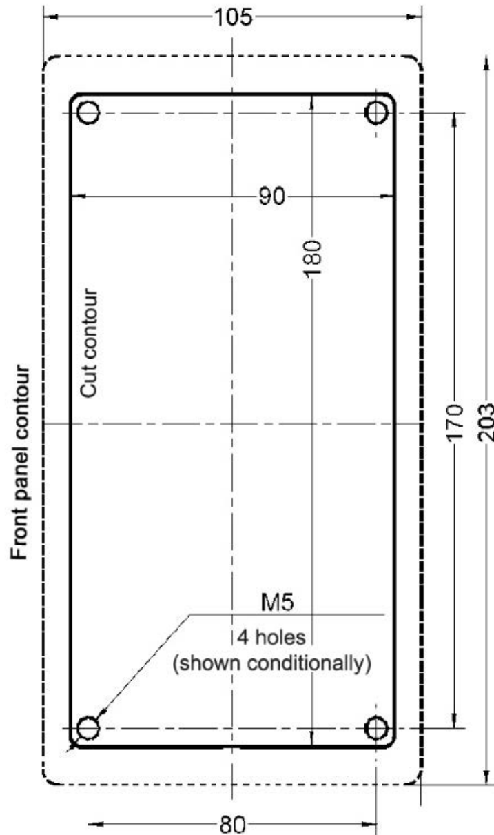
Fig. 1 Markup for installation of the outdoor panel
