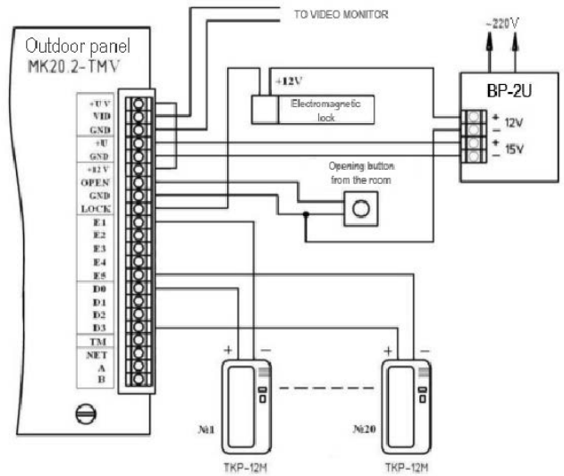
Fig. 2 Example of mounting the outdoor panel MK20.2-TMV
