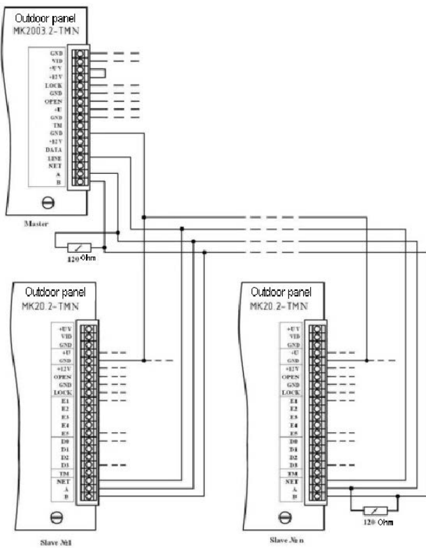
Fig. 3 An example of installation when combining intercoms in a network.
