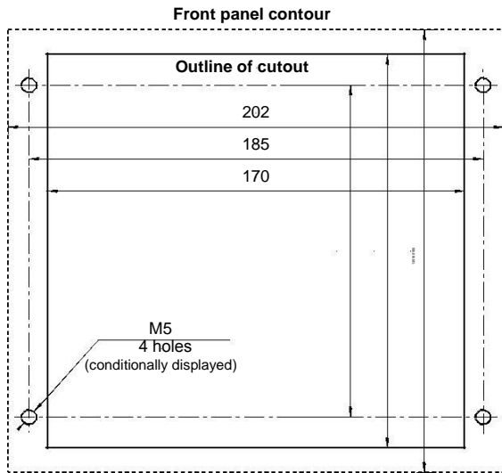
Fig. 1. Markup for the installation of the outdoor panel.
