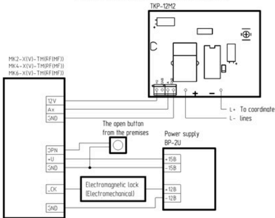
Fig. 2. Scheme of connection of the TKP-12M2 to the four-wire communication line (supply of the handset from the outdoor panel).
