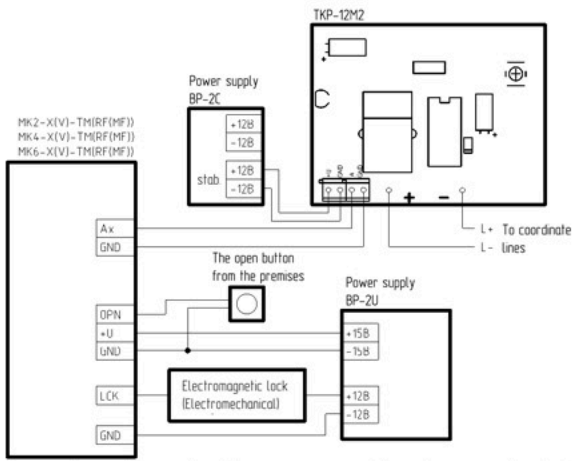
Fig. 1. Scheme of connecting the TKP-12M2 to a four-wire communication line (external power supply for the handset).
